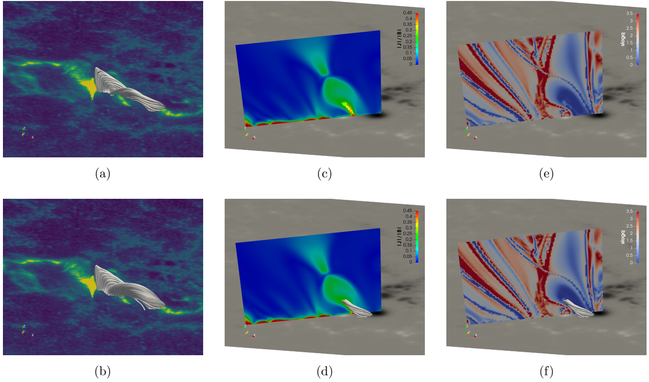
Figure 7. The enlarged and side views of the identified MFR in Figure 6b for the criteria of (a) |T_w| > 1 , and (b) |T_w| > 0.8 , respectively, and similarly for Figure 6c: (c) the distribution of |\mathbf{J}|/|\mathbf{B}| as indicated by the colorbar on a vertical slice across the identified MFR for |T_w| > 1 with the MFR field-line intersection points colored by the corresponding values according to the colorbar, (d) same as (c) but overlotted with the MFR field lines, and (e-f) the distributions of the squashing degree Q on the same slices as (c) and (d).
