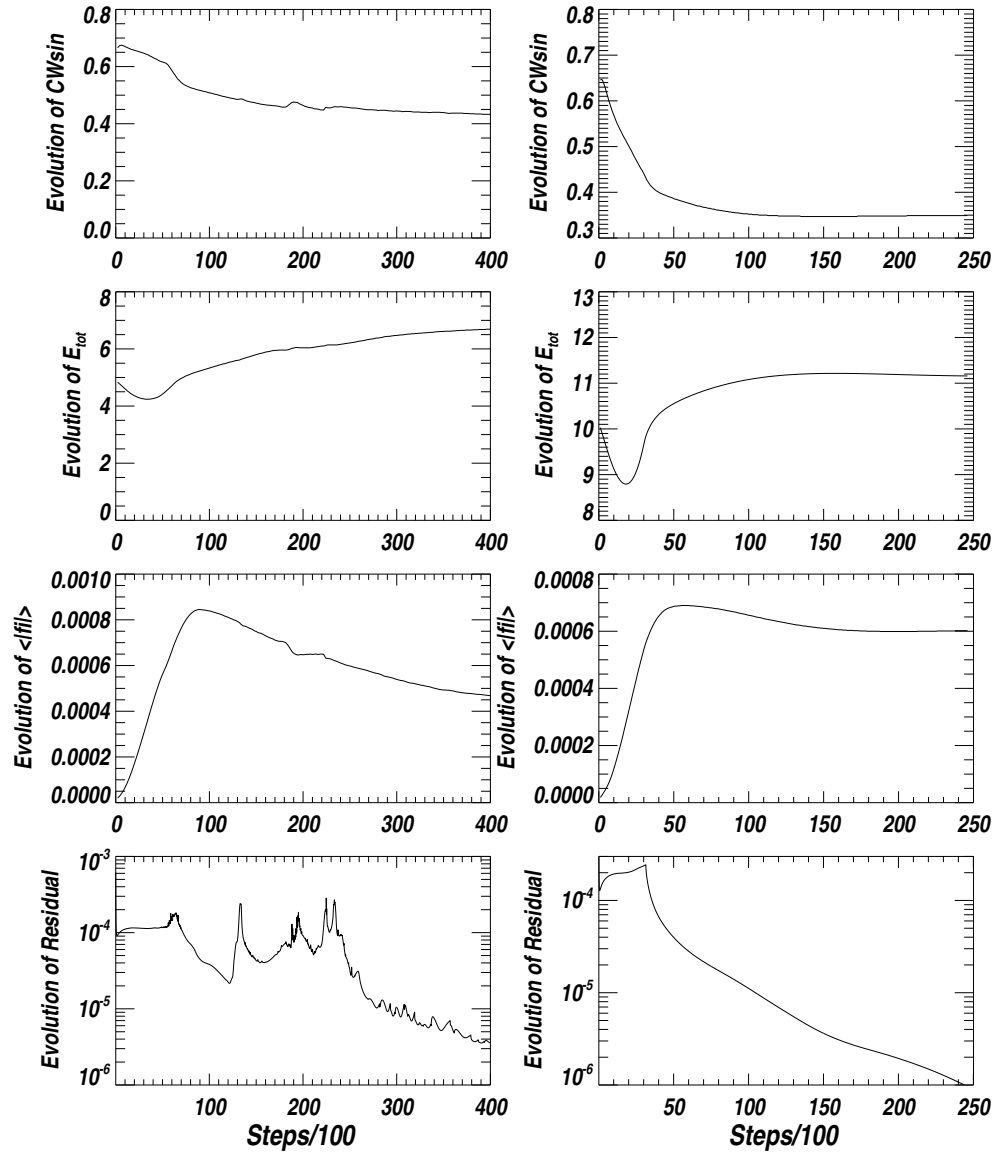
Figure 3. Two sets of convergence metrics of two extrapolation runs for AR11719 (event 1, left column) and AR12158 (event 2, right column). The top three rows show the metrics of CW_{sin} , the total magnetic energy E_{tot} (arbitrary unit), and \langle |f_i| \rangle , respectively. Panels in the bottom row show the evolution of residuals for the two events.
